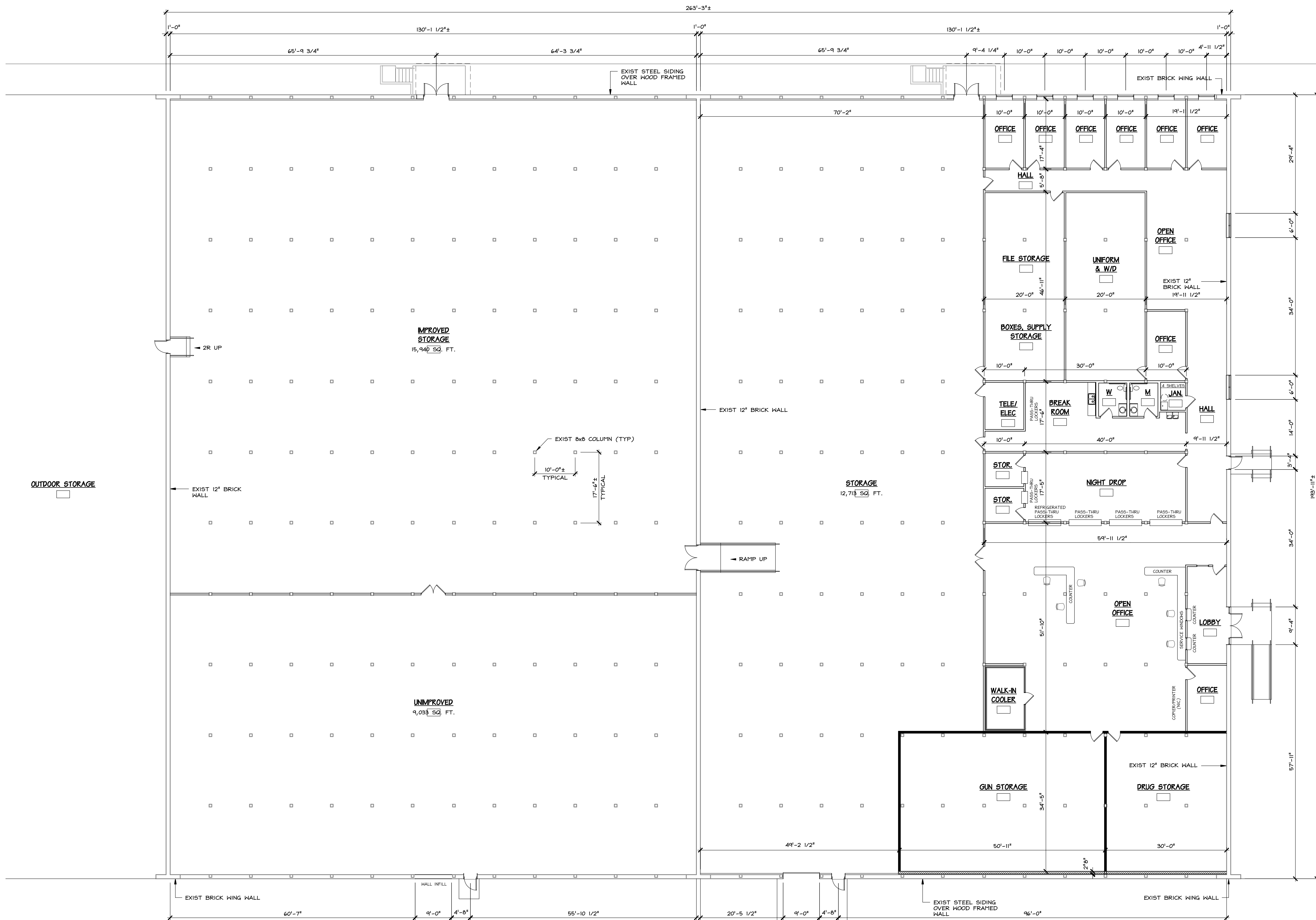
FLOOR PLAN SCALE: 3/32" = 1'-0"
